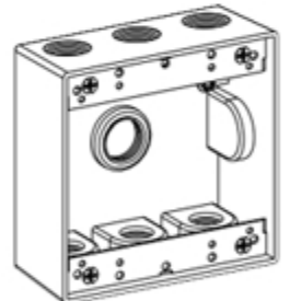
GTGB50-7 GTGB75-7
